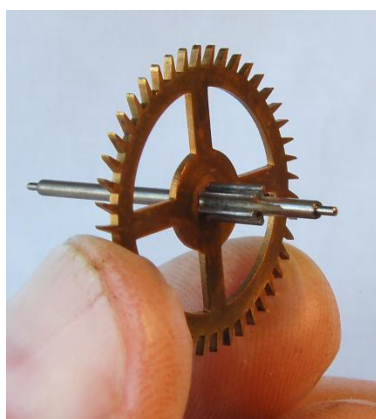
Figure 87 – escape wheel and pinion
