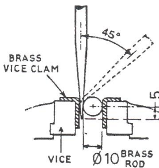
Figure 141 – bend in vice
