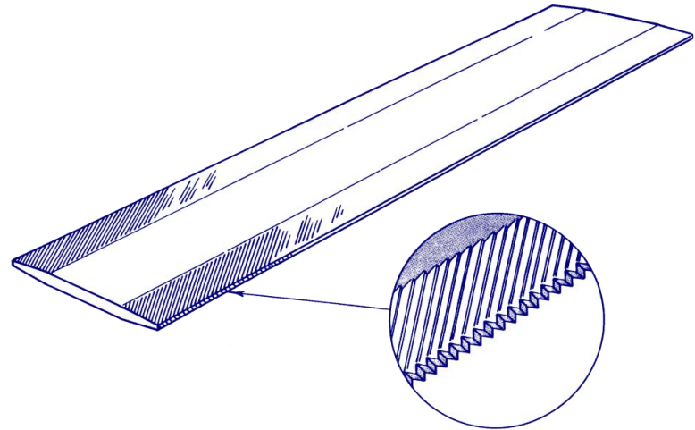
Figure 127 – slotting file
