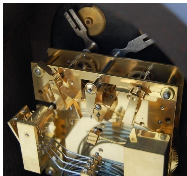
Figure 31 – another view (note the platform escapement mounted between the plates)
