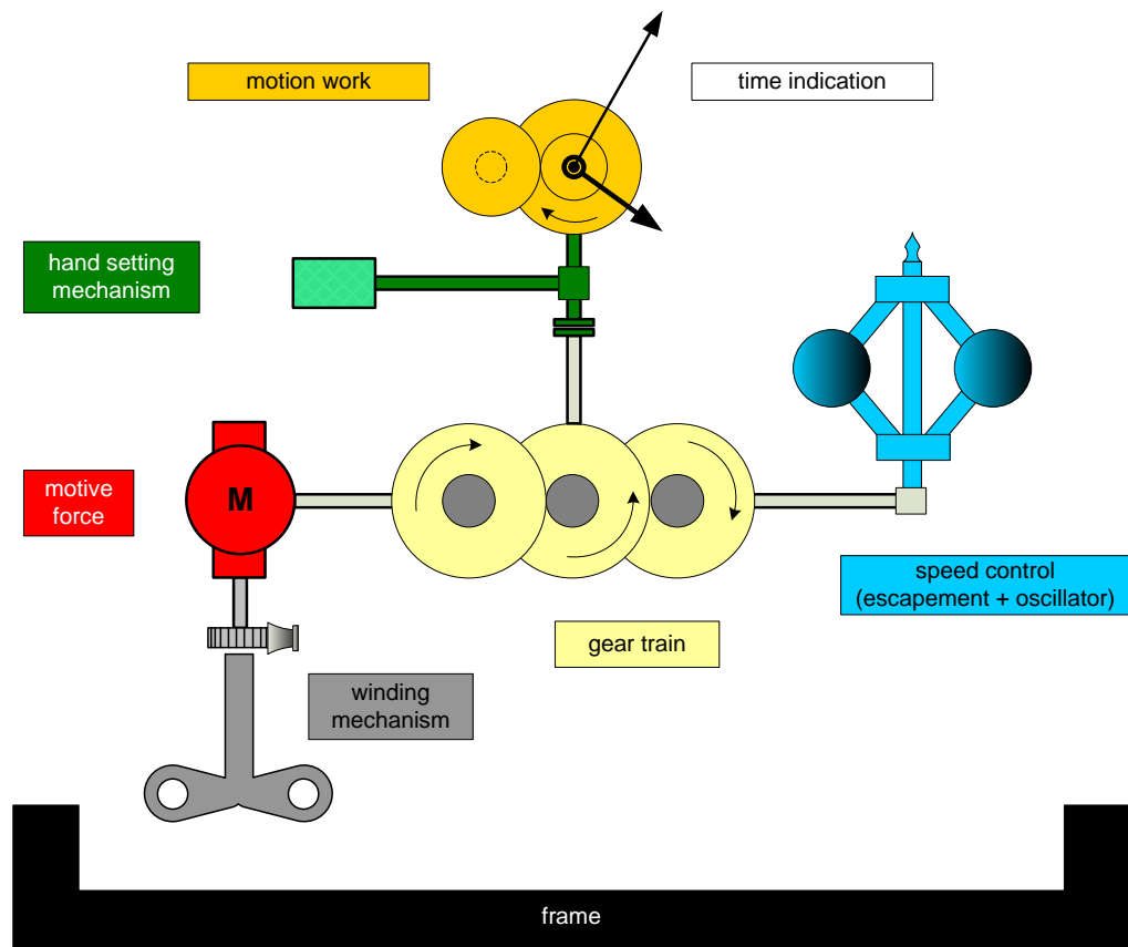
Figure 55 – the divisions of a mechanical movement
