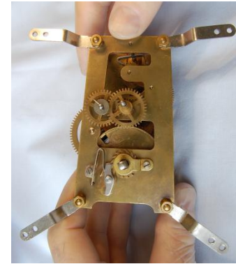
Figure 58 – front view of movement
