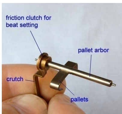
Figure 69 – pallet assembly
