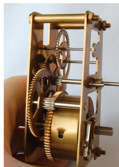
Figure 77 – another view of the train
