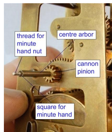
Figure 63 – centre arbor and cannon pinion
