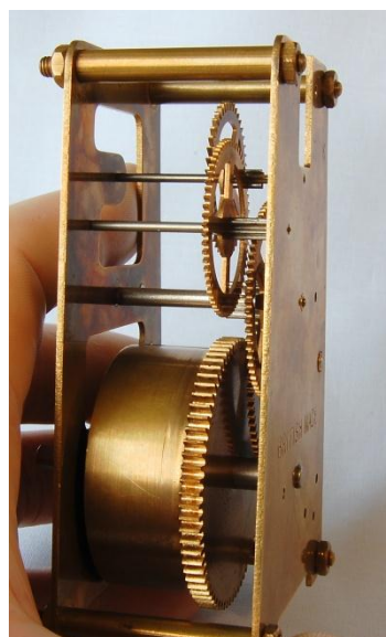
Figure 76 – the train in position
