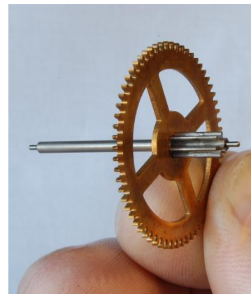
Figure 86 – third wheel and pinion
