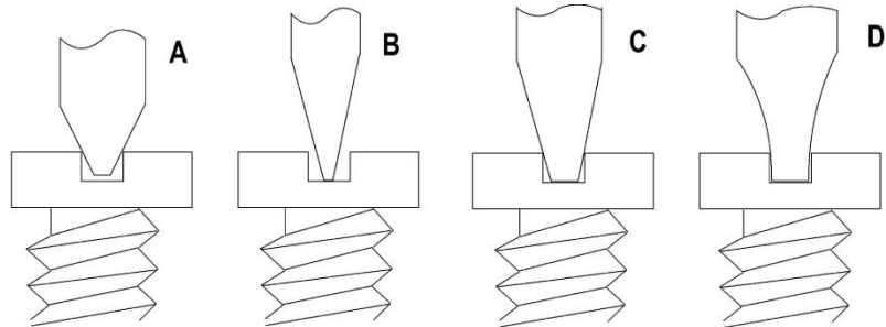
Figure 107 – the screwdriver blade must be the right angle and width for the slot
